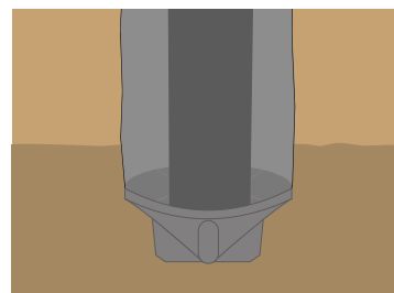
Pile shoe grouted
